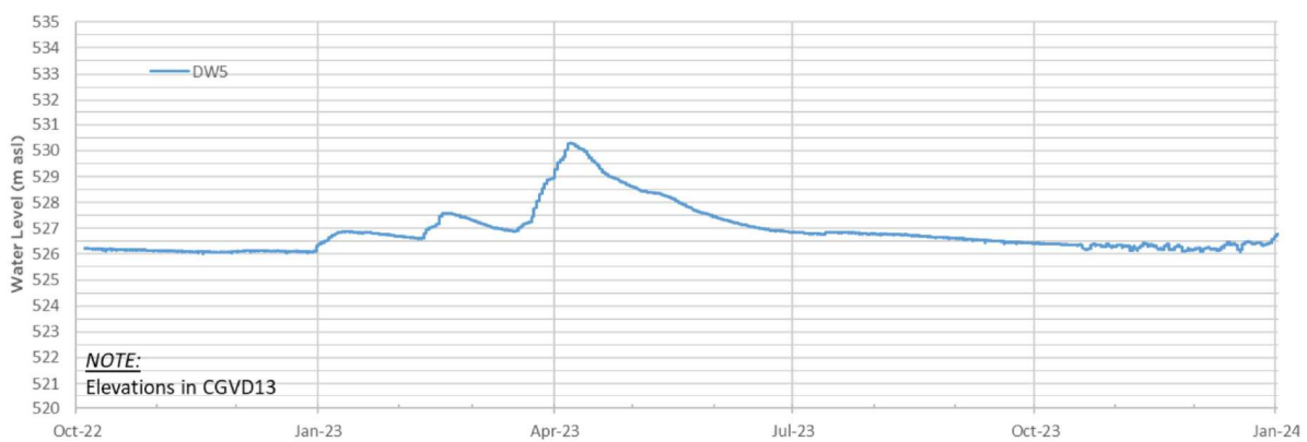
Figure B.50: Hydrograph of water levels at Domestic Well DW5, masl.
